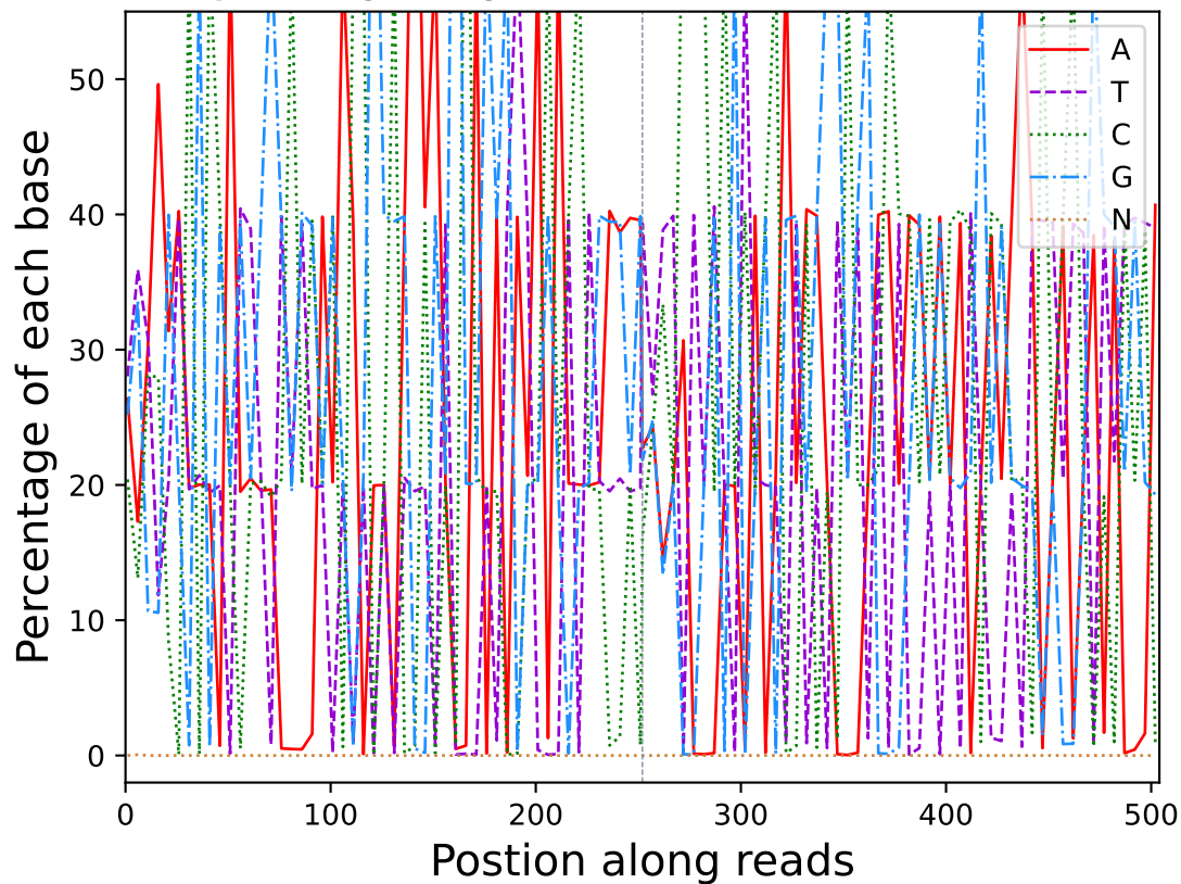
Base percentage along reads (R10326)
